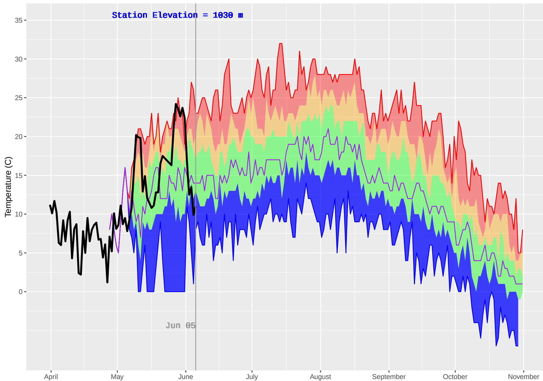
WITCH (154) : Historical (1993–2018) and Current (2019) Daily Temperature
