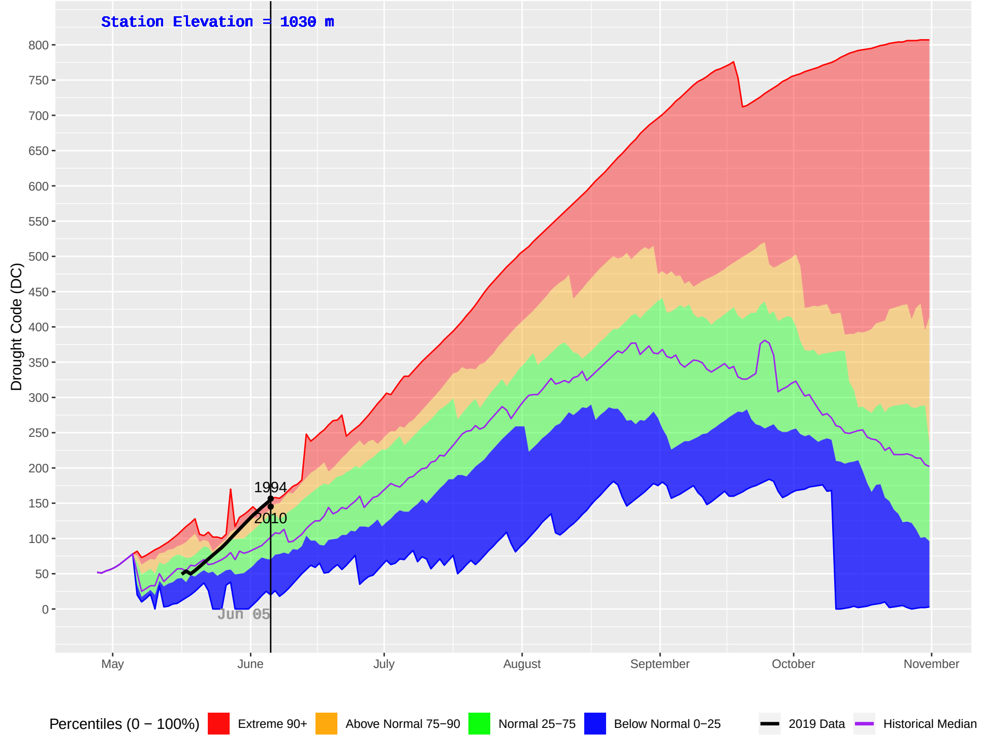
WITCH (154) : Historical (1993–2018) and Current (2019) Daily Drought Code (DC)
