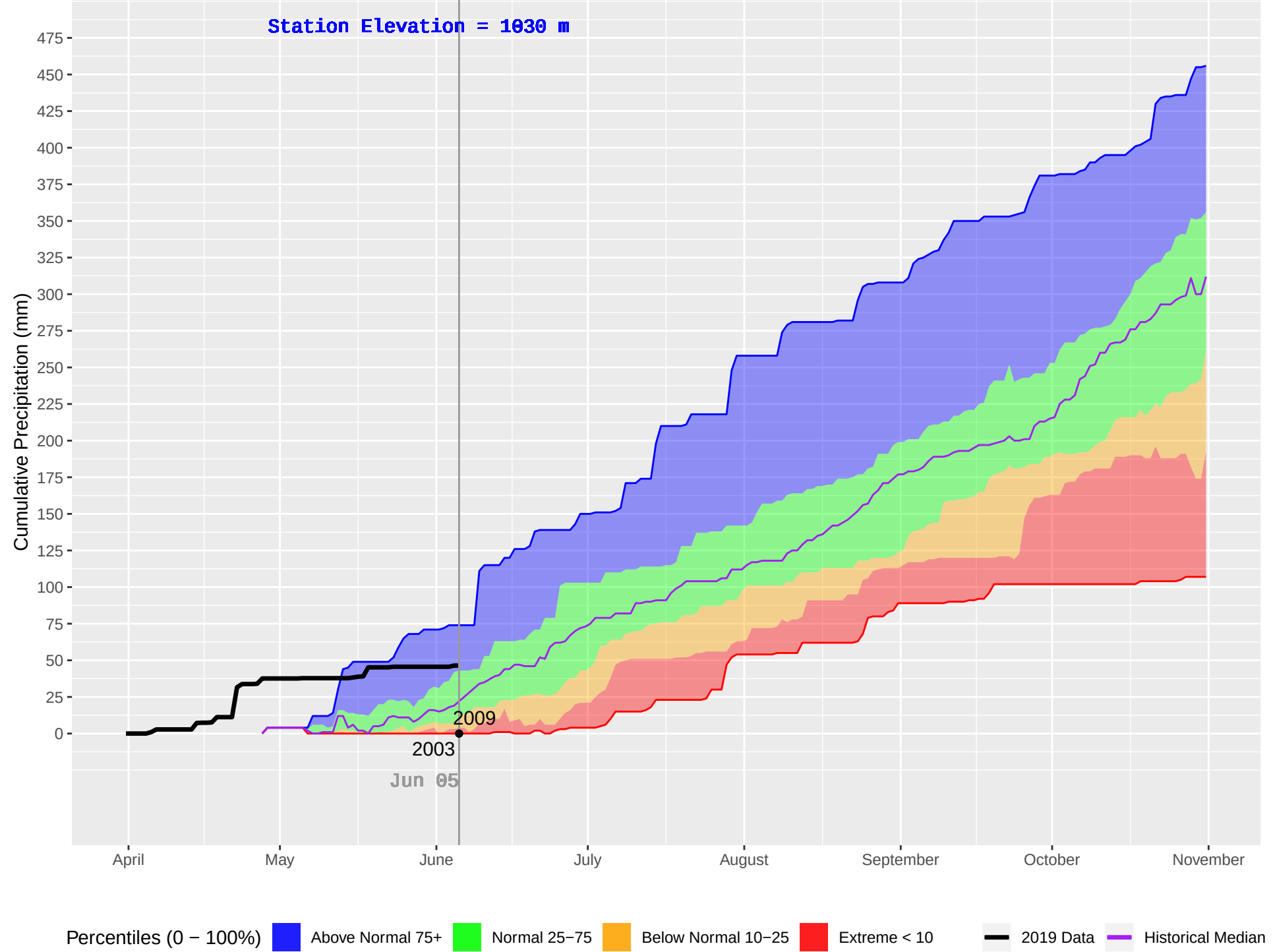
WITCH (154) : Historical (1993–2018), Current (2019) Daily Cumulative Precipitation
