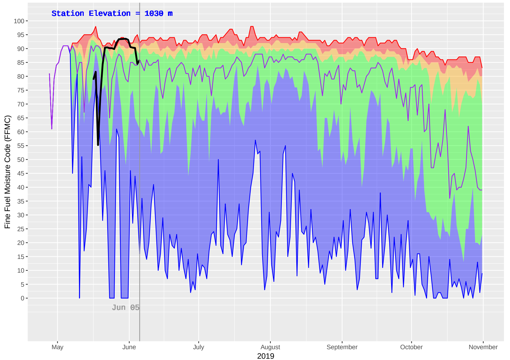
WITCH (154) : Historical (1993–2018) and Current (2019) Daily Fine Fuel Moisture Code (FFMC)
