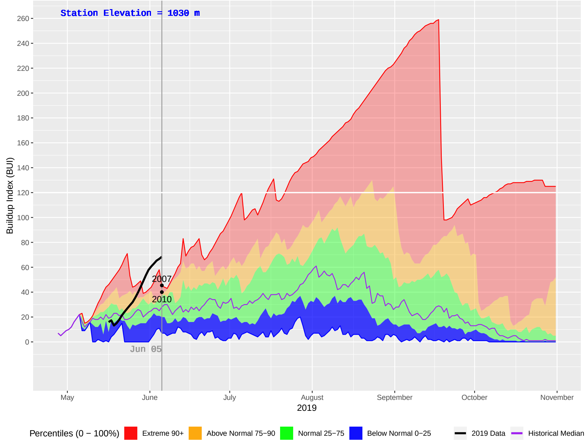
WITCH (154) : Historical (1993–2018), Current (2019) Daily Buildup Index (BUI)
