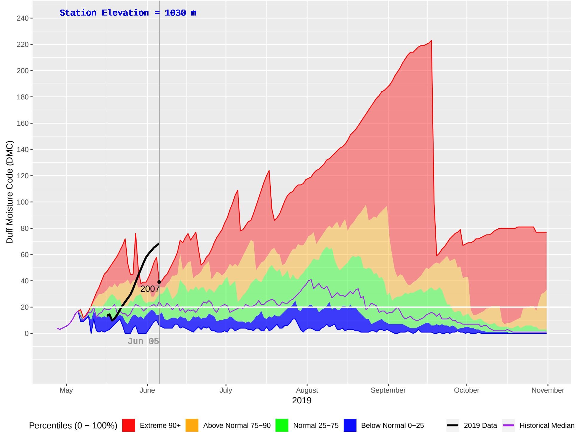
WITCH (154) : Historical (1993–2018), Current (2019) Daily Duff Moisture Code (DMC)
