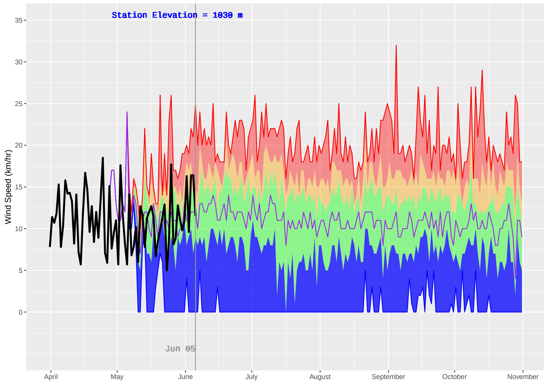
WITCH (154) : Historical (1993–2018) and Current (2019) Daily Wind Speed
