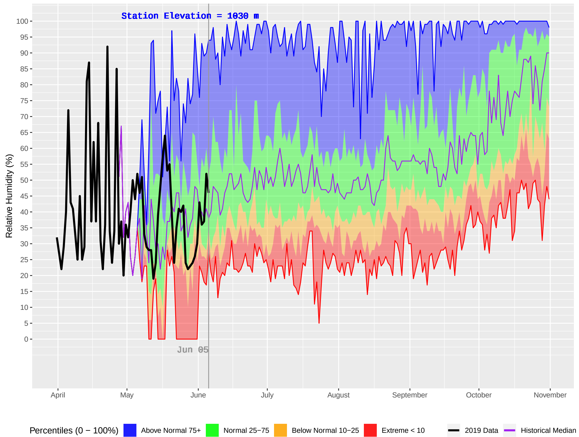
WITCH (154) : Historical (1993–2018) and Current (2019) Daily Relative Humidity
