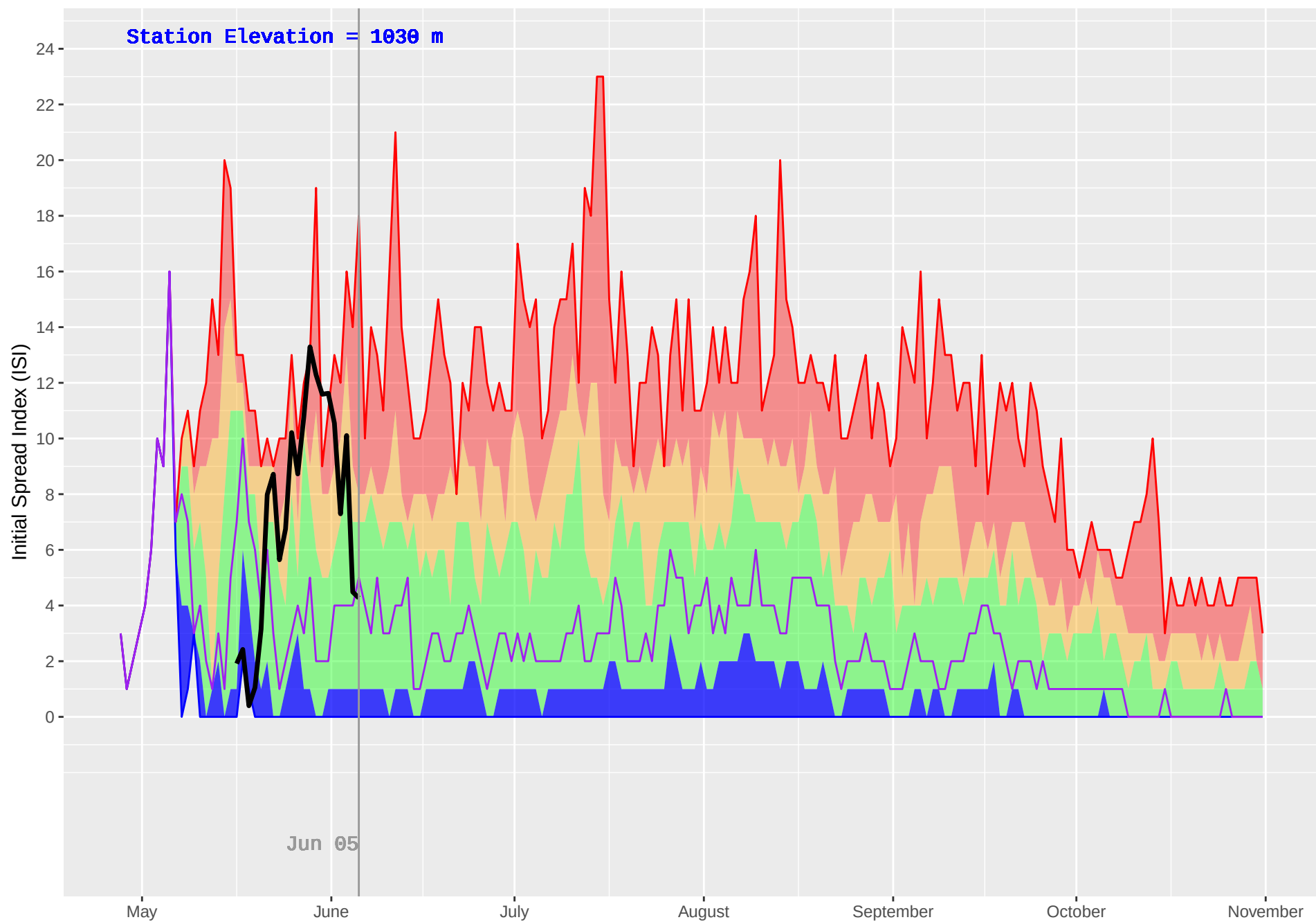
WITCH (154) : Historical (1993–2018) and Current (2019) Daily Initial Spread Index (ISI)
