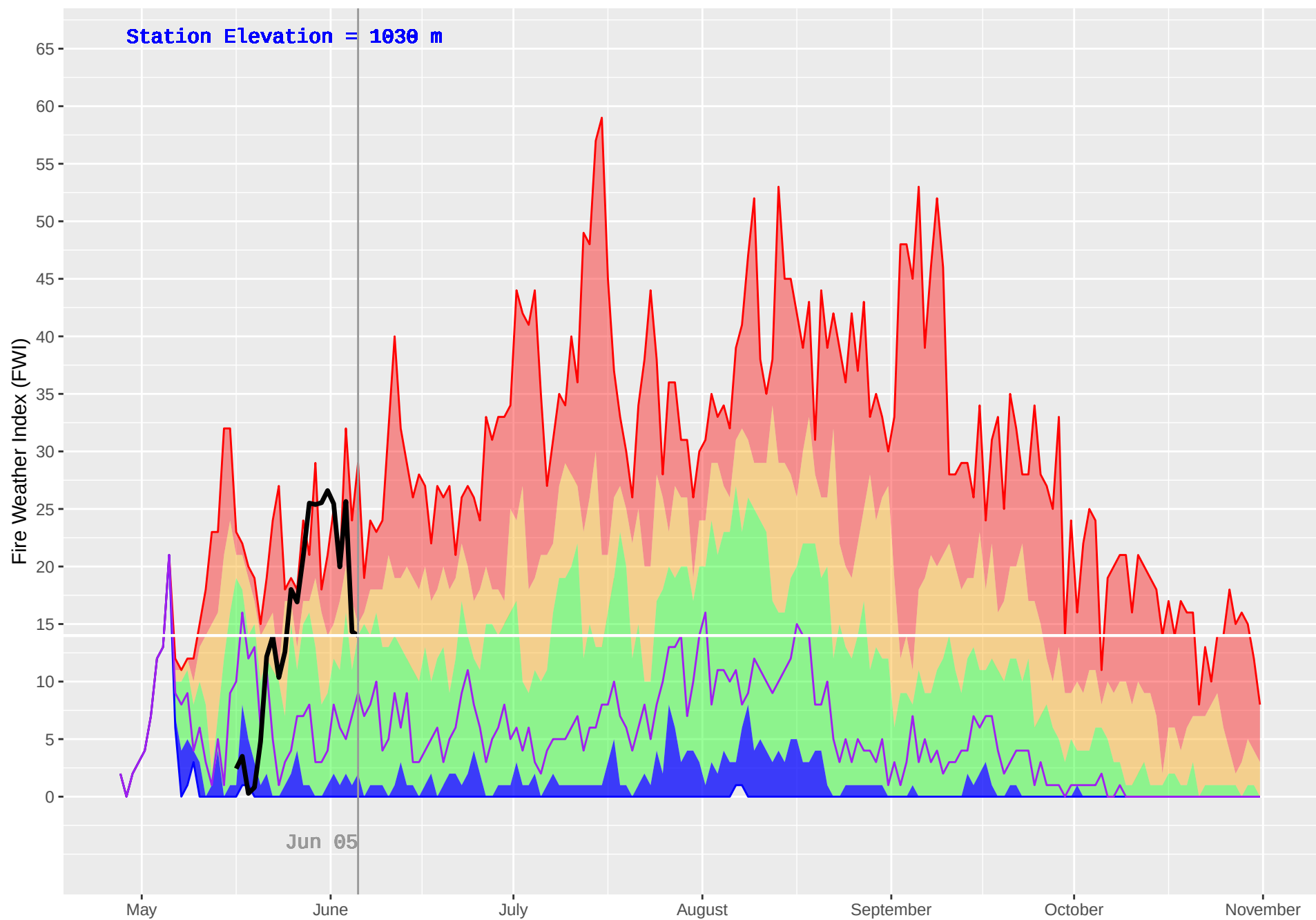
WITCH (154) : Historical (1993–2018) and Current (2019) Daily Fire Weather Index (FWI)
